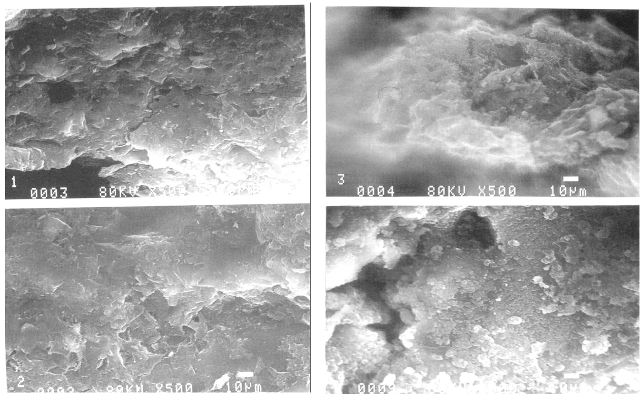
Figure 4-5: SEM Photographs of mortar and series
